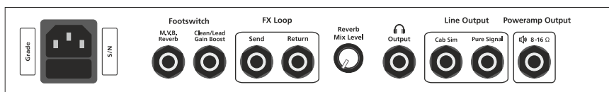
Figure: Back panel E606 head
